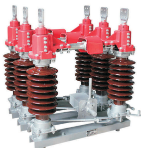
GW4-40.5
