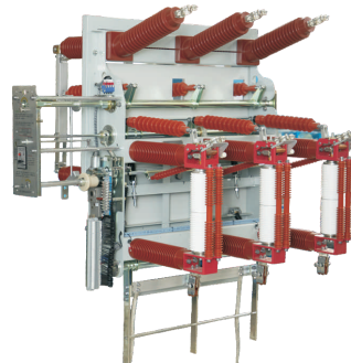
FZ(R)N21-40.5G
