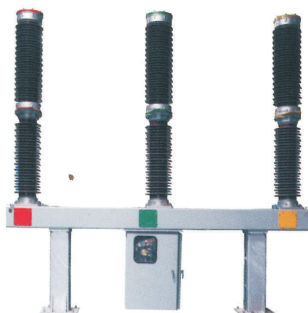
LW36A-126/145
