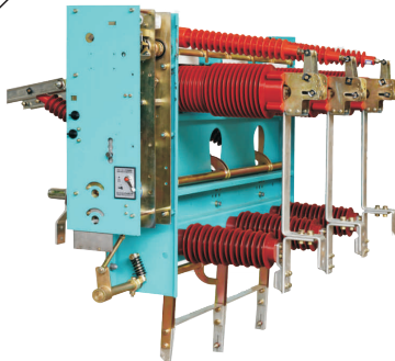
LQGF-40.5ZD
