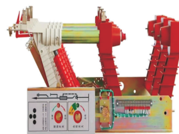
FKRN12-24(D)/125-31.5
